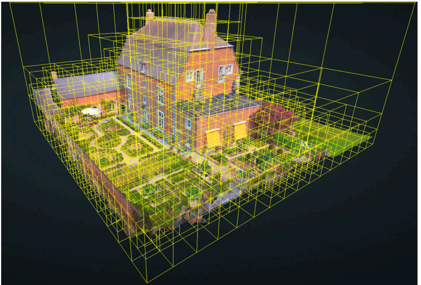
Cube structure of the octree @Potree
